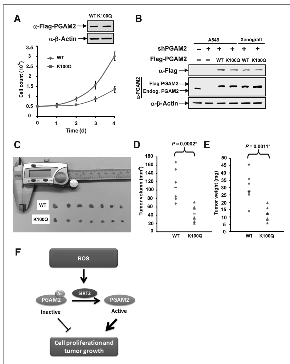
Figure 7. Acetylation mimetic K100Q mutant inhibits cell proliferation and tumor growth. A , acetylation mimetic mutant K100Q suppresses cell proliferation. A total of 5 \times 10^4 indicated stable cells were seeded in each well. Cell numbers were counted every 24 hours. Error bars represent cell numbers \pm SD for triplicate experiments. B , the expression of PGAM2 and PGAM2 K100Q in stable cell lines and xenograft tumors. Whole-cell extracts were prepared from either original A549 stable cell pools or xenograft tumors, followed analysis by Western blotting. C , acetylation mimetic mutant K100Q inhibits xenograft tumor growth in vivo . Nude mice were injected with A549 PGAM2 cells or PGAM2 K100Q cells. The xenograft tumors were dissected and measured after 7 weeks and shown. D and E , quantification of average volume and weight of xenograft tumors are shown in D and E , respectively. Error bars represent \pm SD for 7 tumors.
