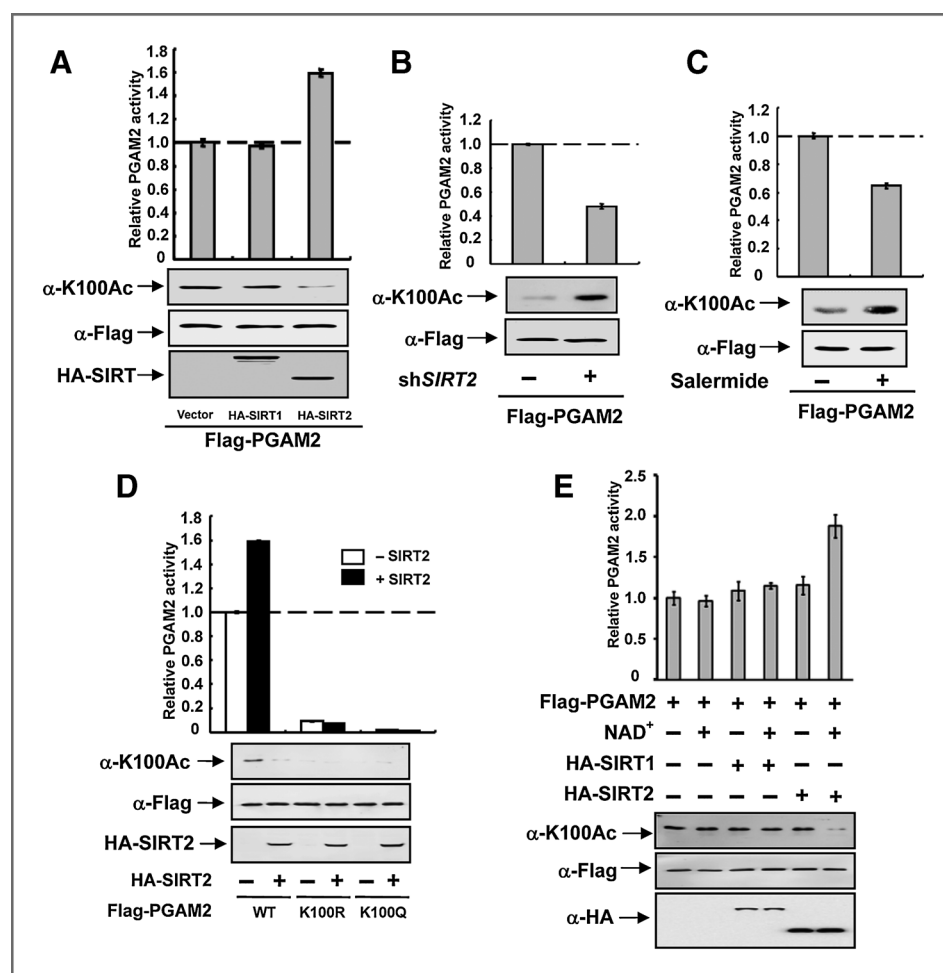
Figure 4. SIRT2 activates PGAM2. A , SIRT2 increases PGAM2 activity. HEK293T cells were transfected with indicated plasmids, Flag-PGAM2 was immunoprecipitated, and PGAM2 activity was assayed. Mean values of relative enzyme activity of triplicate experiments with \pm SD are presented. B , SIRT2 knockdown decreases PGAM2 activity. Scramble and SIRT2 knocking-down stable HEK293T cells were transfected with Flag-PGAM2, and PGAM2 protein was immunoprecipitated and activity was assayed. Error bars represent \pm SD for triplicate experiments. C , inhibition of SIRT2 decreases PGAM2 activity. HEK293T cells were transfected with Flag-PGAM2, followed by treatment with salermide. Flag-PGAM2 was immunoprecipitated, and PGAM2 activity was measured. Relative enzyme activities of triplicate experiments \pm SD are presented. D , SIRT2 overexpression does not activate K100 mutants of PGAM2. WT and mutant PGAM2 were co-expressed in HEK293T cells with SIRT2, respectively, and purified by Flag beads, followed by enzyme assay and Western blotting. The mean value of triplicates and \pm SD are presented. E , SIRT2 deacetylates and activates PGAM2 in vitro . Flag-PGAM2, HA-SIRT1, and HA-SIRT2 were purified from HEK293T cells, respectively, and the in vitro deacetylation assay was performed as described. Samples were determined by Western blotting with indicated antibodies.
