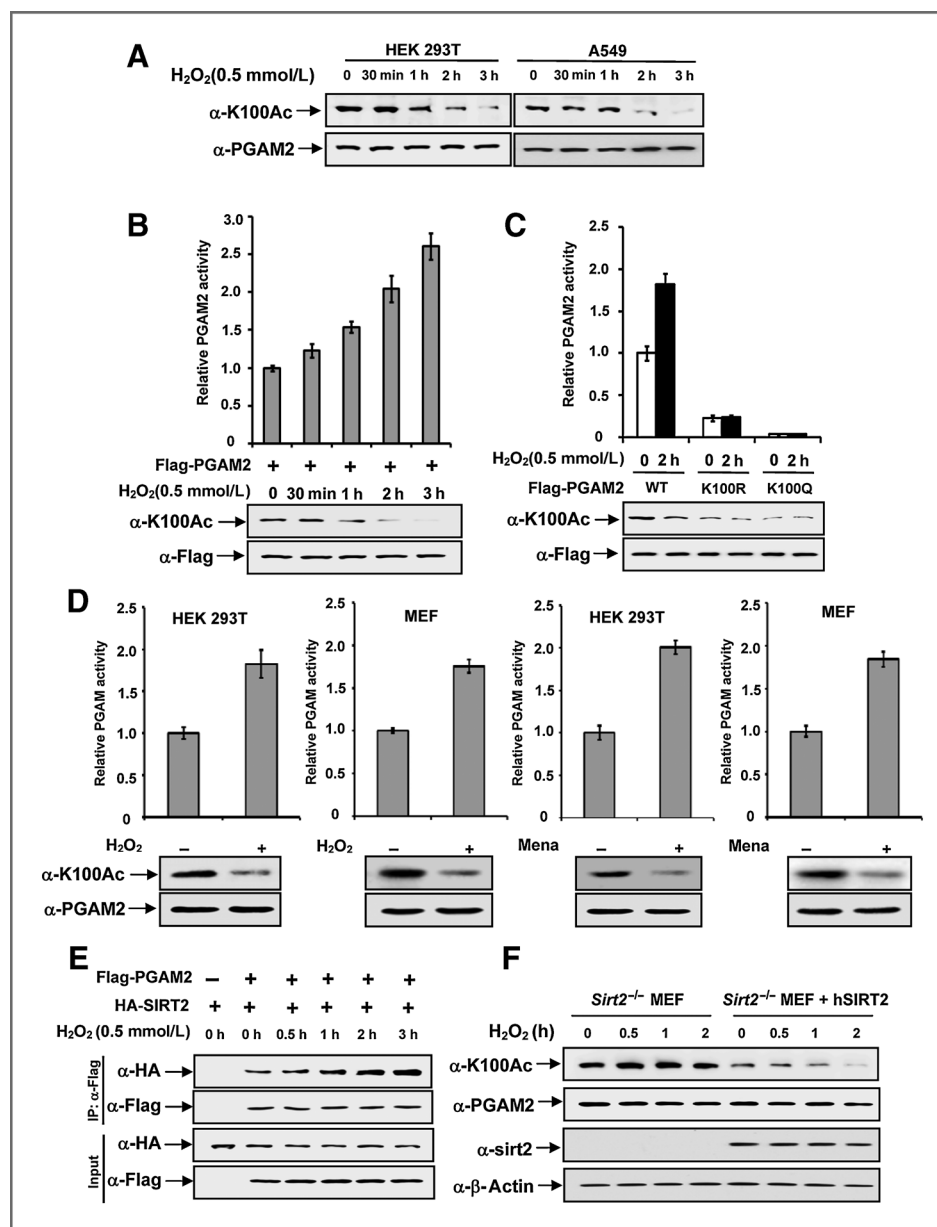
Figure 5. Oxidative stress decreases K100 acetylation levels and induces PGAM2 activity. A , H_2O_2 treatment decreases endogenous K100 acetylation level. HEK293T and A549 cells were treated with H_2O_2 for different lengths of time as indicated. The levels of K100 acetylation were determined by Western blotting with anti-acetyl-PGAM2 (K100) antibody. B , H_2O_2 -induced oxidative stress increases PGAM2 activity. HEK293T cells were transfected with Flag-PGAM2 and then treated with H_2O_2 for indicated time, followed by immunoprecipitation, and enzyme activity was measured and normalized against protein levels. Mean values of relative enzyme activity of triplicate experiments with \pm SD are presented. C , H_2O_2 increases WT PGAM2 activity, but not K100 mutants. HEK293T cells were transfected with indicated plasmids, followed by H_2O_2 treatment for 2 hours, immunoprecipitated, and then PGAM2 activity was assayed. Relative enzyme activities of triplicate experiments \pm SD are presented. D , oxidative stress increases the endogenous PGAM activity via reducing the K100 acetylation level. HEK293T cells or WT MEF cells were treated with H_2O_2 for 2 hours or Menadione (Mena) for 30 minutes, respectively, and then endogenous PGAM activity was assayed. The K100 acetylation levels of PGAM2 were determined by Western blot analysis. Relative enzyme activities of triplicate experiments \pm SD are presented. E , oxidative stress increases the interaction between SIRT2 and PGAM2. HEK293T cells were transfected with indicated plasmids, and the SIRT2-PGAM2 association was examined by immunoprecipitation (IP)-Western blot analysis. F , Sirt2 mediates K100 deacetylation in response to oxidative stress. Sirt2 -/- MEFs and Sirt2 -/- MEFs stably expressing human SIRT2 were treated with H_2O_2 for indicated time. The change of K100 acetylation levels of PGAM2 was determined by Western blot analysis.
