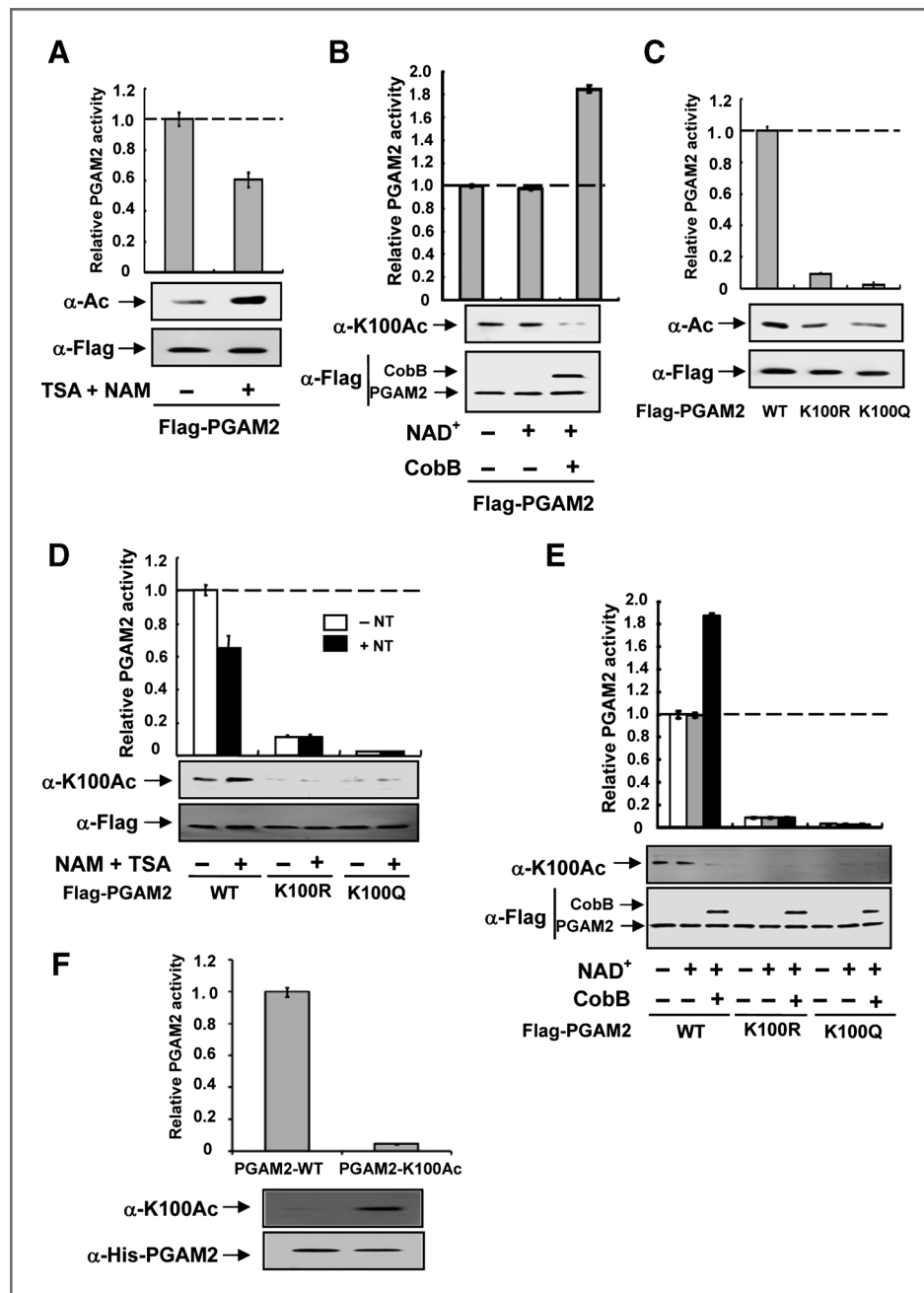
Figure 2. Acetylation at K100 reduces PGAM2 activity. A , inhibition of deacetylases decreases PGAM2 enzyme activity. Flag-tagged PGAM2 was expressed in HEK293T cells, which were treated with or without TSA and NAM, followed by immunoprecipitation, and enzyme activity was measured and normalized against protein levels. The protein levels and acetylation levels were determined by Western blotting. Mean values \pm SD of relative enzyme activity of triplicate experiments are presented. B , PGAM2 is activated by in vitro deacetylation. Flag-PGAM2 was expressed in HEK293T cells, purified, and incubated with recombinant CobB. Samples were analyzed for acetylation levels and PGAM2 enzyme activity. Relative enzyme activities of triplicate experiments \pm SD are presented. C , K100 mutation decreases PKM2 enzyme activity. Flag-tagged WT and mutant PGAM2 proteins were expressed in HEK293T cells and purified by immunoprecipitation. The enzyme activity was measured and normalized against protein level. Error bars represent \pm SD for triplicate experiments. D , inhibition of deacetylases with TSA and NAM treatment decreases the activity of WT, but not K100-mutant PGAM2. Flag-tagged WT and mutant PGAM2 proteins were expressed in HEK293T cells, followed by treatment with TSA and NAM, and then purified by immunoprecipitation. The PGAM2 enzyme activity was measured and normalized against protein level. The mean value of triplicates and \pm SD are presented. E , WT PGAM2, but not K100-mutant PGAM2, is activated by in vitro deacetylation. Flag-tagged WT and mutant PGAM2 proteins were expressed in HEK293T cells, then purified and incubated with recombinant CobB, followed by enzyme activity assay. Relative enzyme activities of triplicate experiments \pm SD are presented. F , K100-acetylated PGAM2 has lower enzyme activity. Recombinant WT and K100-acetylated PGAM2 protein were purified in E. coli . The enzyme activity was measured and normalized against protein level. Mean values of relative enzyme activity of triplicate experiments with \pm SD are presented.
