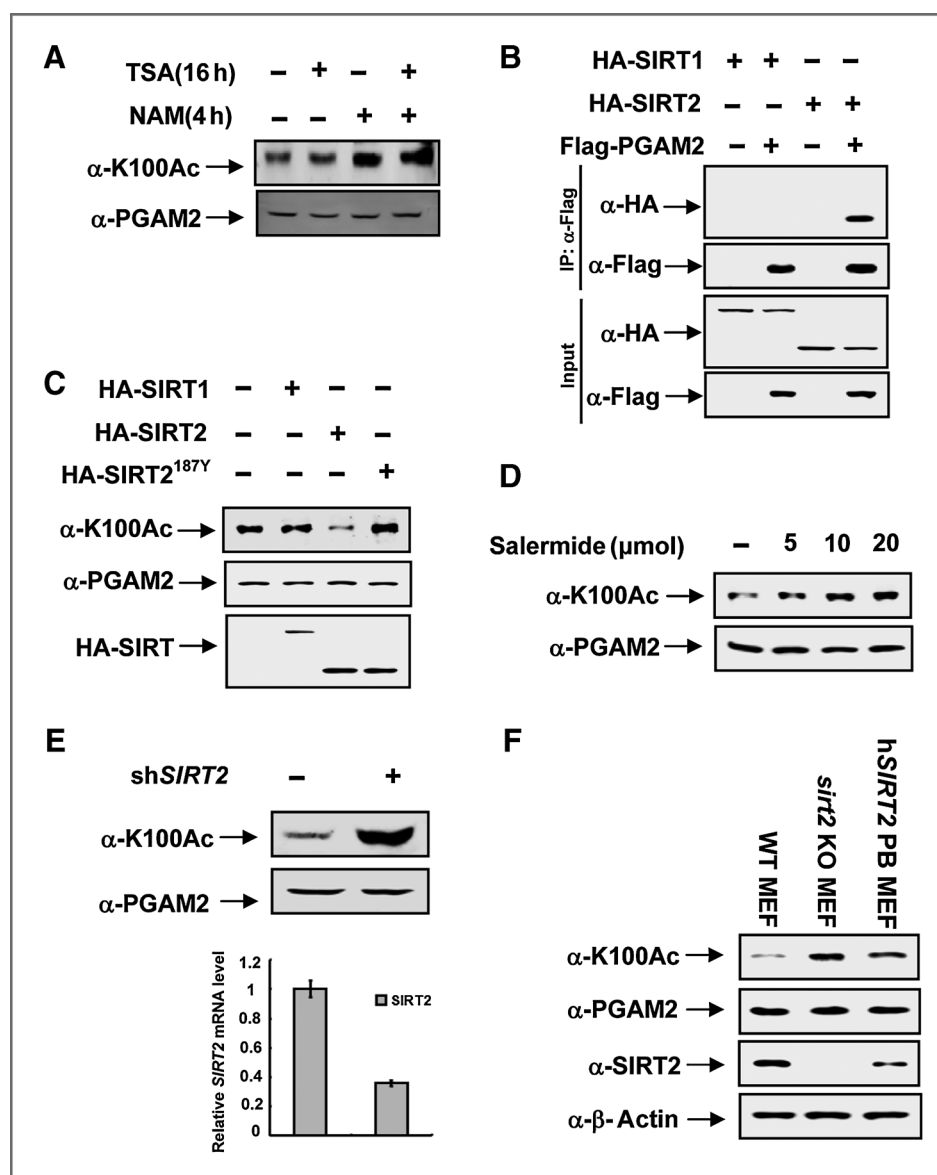
Figure 3. SIRT2 deacetylates PGAM2 at K100. A , NAM, but not TSA, increases PGAM2 K100 acetylation. HEK293T cells were treated with either NAM or TSA, endogenous PGAM2 protein and K100 acetylation levels were determined by Western blotting with PGAM2 antibody or anti-acetyl-K100 antibody, respectively. B , SIRT2 interacts with PGAM2. HEK293T cells were transfected with indicated plasmids, and interactions between PGAM2 and SIRT1 or SIRT2 were examined by immunoprecipitation and Western blot analysis. C , WT SIRT2 overexpression decreases PGAM2 K100 acetylation. K100 acetylation levels of PGAM2 in HEK293T cells expressing indicated plasmids were detected by Western blotting. D , salermide, the SIRT2 inhibitor, increases the K100 acetylation of PGAM2. HEK293T cells were cultured at different concentrations of salermide. The K100 acetylation levels were probed by anti-acetyl-K100 antibody. E , knocking down SIRT2 increases endogenous K100 acetylation of PGAM2. HEK293T cells were infected with retrovirus targeting SIRT2, and the levels of PGAM2 protein and K100 acetylation were determined by Western blotting. SIRT2 knockdown efficiency was determined by quantitative PCR. Error bars represent \pm SD for triplicate experiments. F , the K100 acetylation level of PGAM2 is increased in sirt2 knockout MEFs and decreased in hSIRT2 put-back MEFs. The indicated cell lysates were prepared, and levels of PGAM2 protein and K100 acetylation were detected by Western blotting using indicated antibodies.
